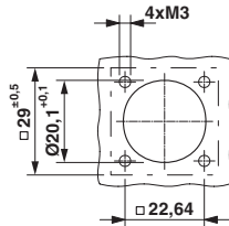
Dimensional drawing
